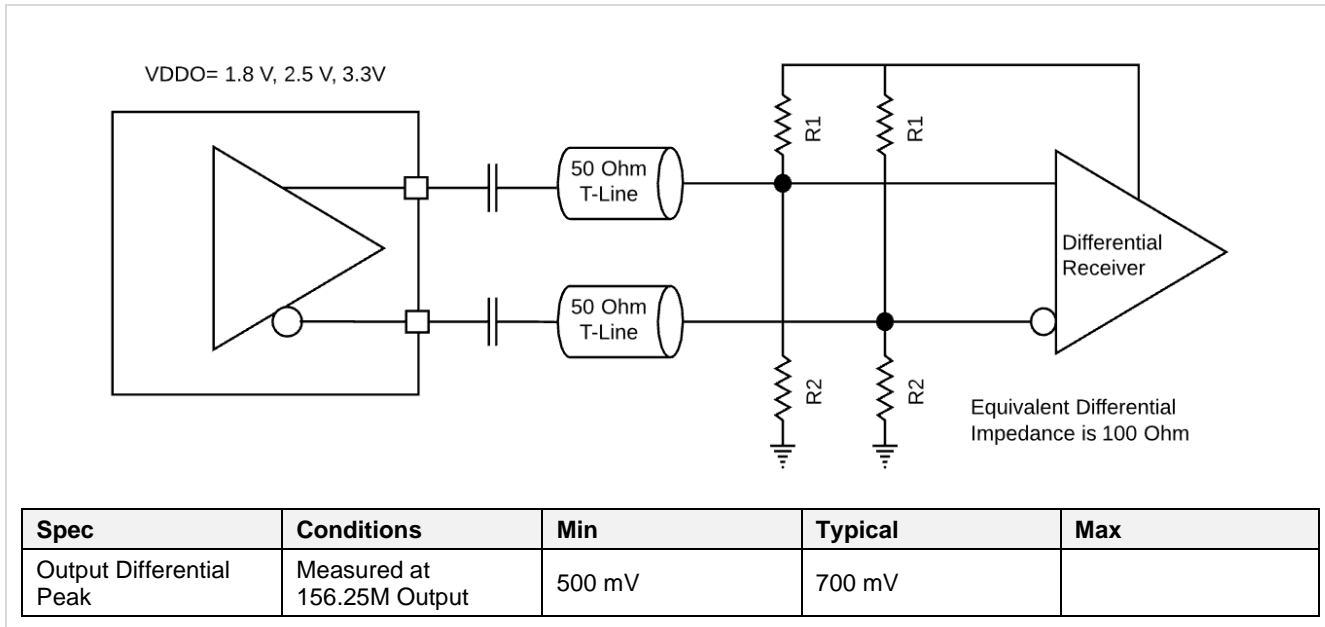
Figure 26. LVDS Boost Standard for the SiT95148 Output Driver with AC Termination at the Load
