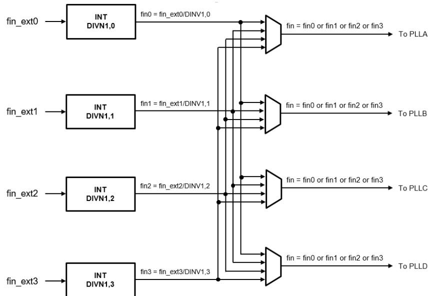
Figure 9. Input Clock Distribution
