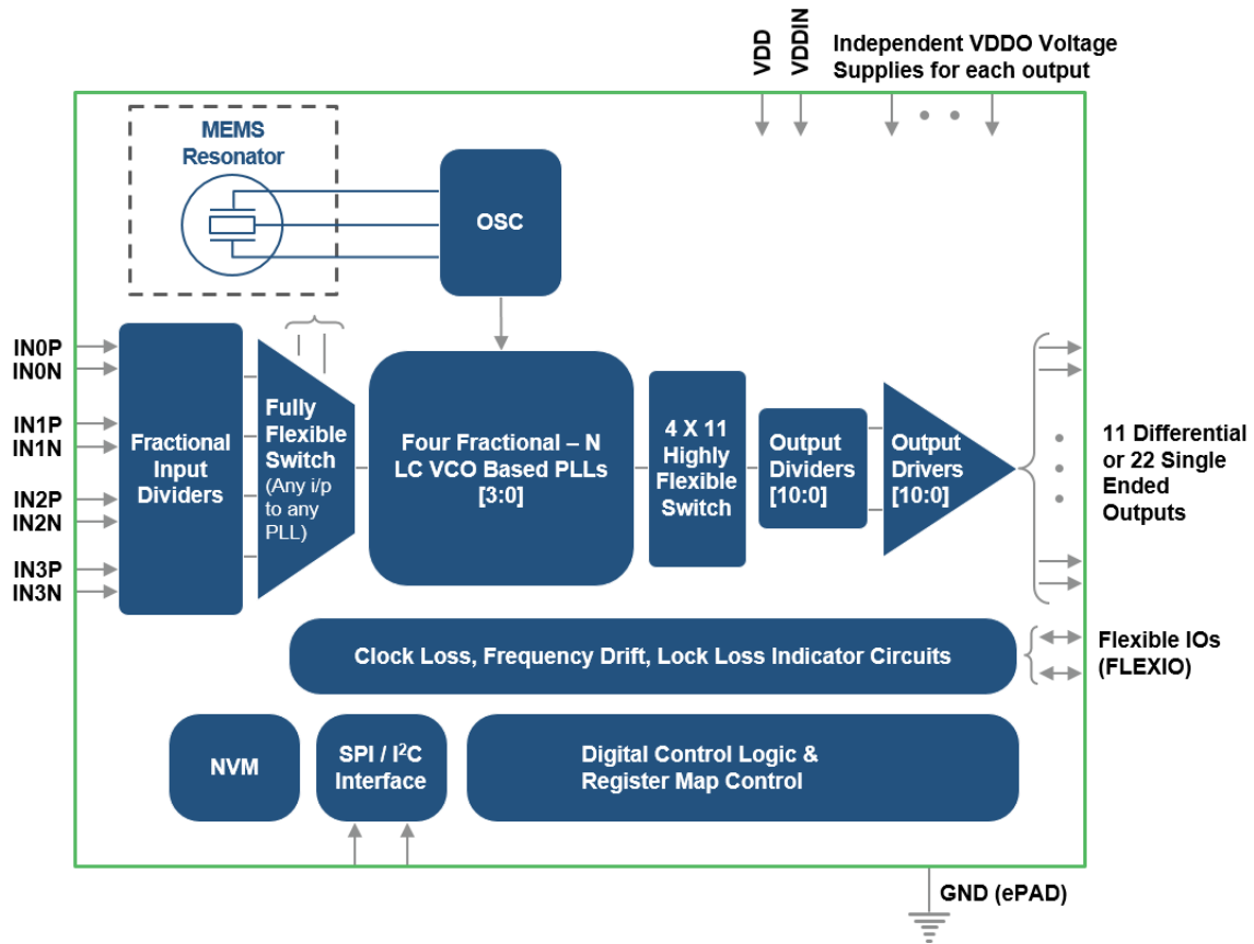
Figure 1. SiT95148 Block Diagram
