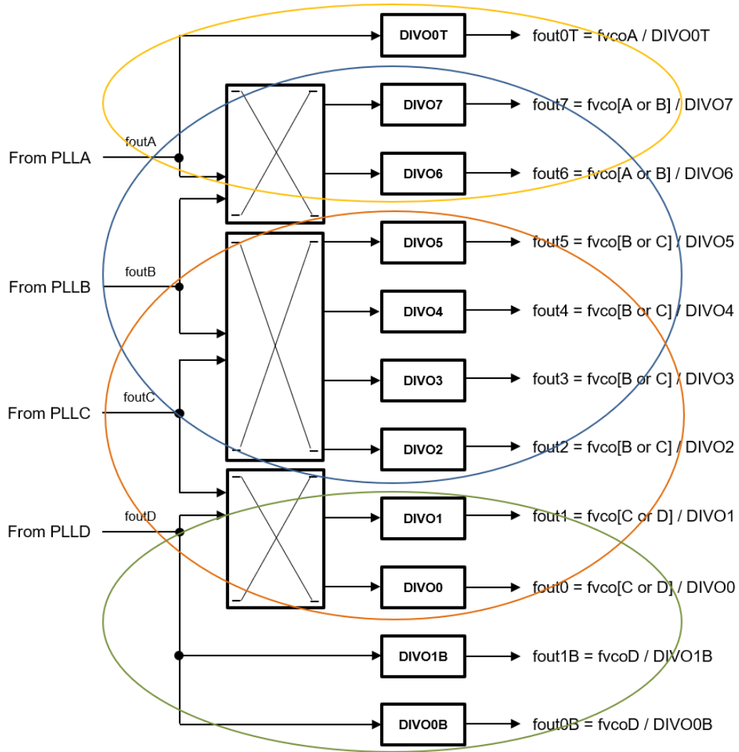
Figure 10. Output Clock Distribution
