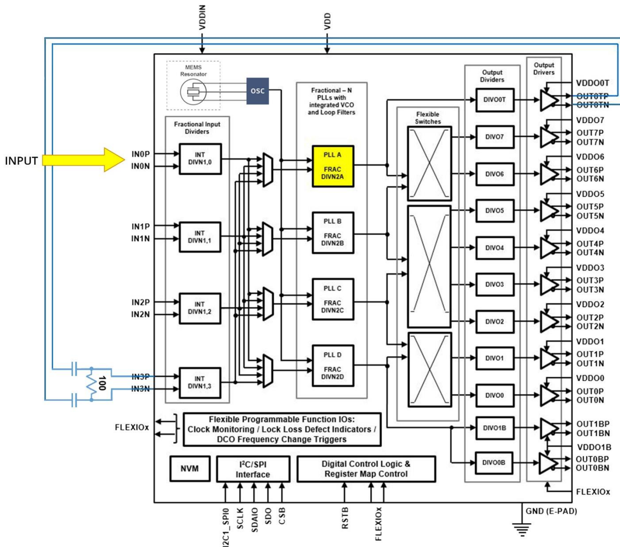
Figure 30. SiT95148 Zero Delay Mode Setup
