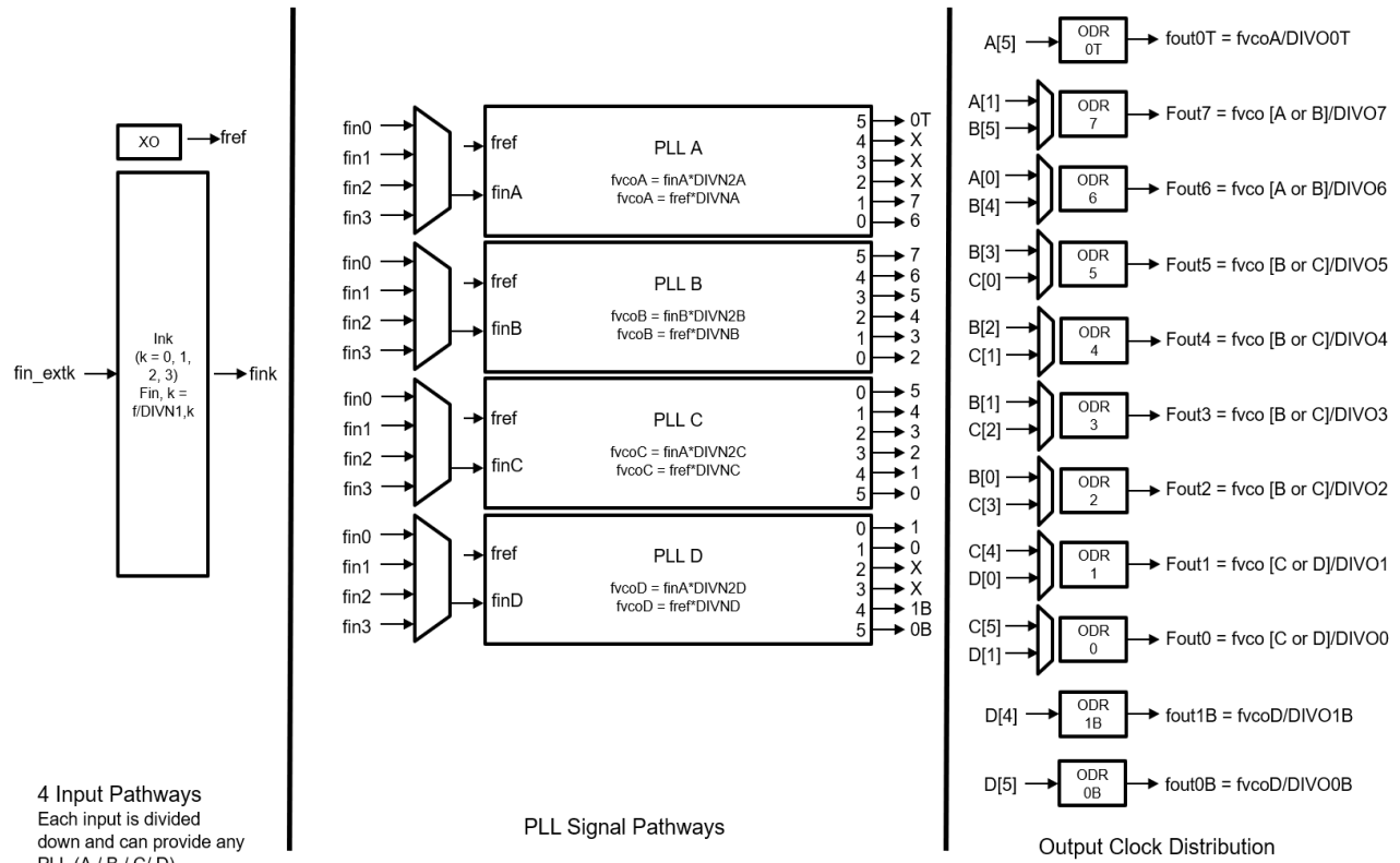
Figure 8. Overall Hierarchy of Clocks
