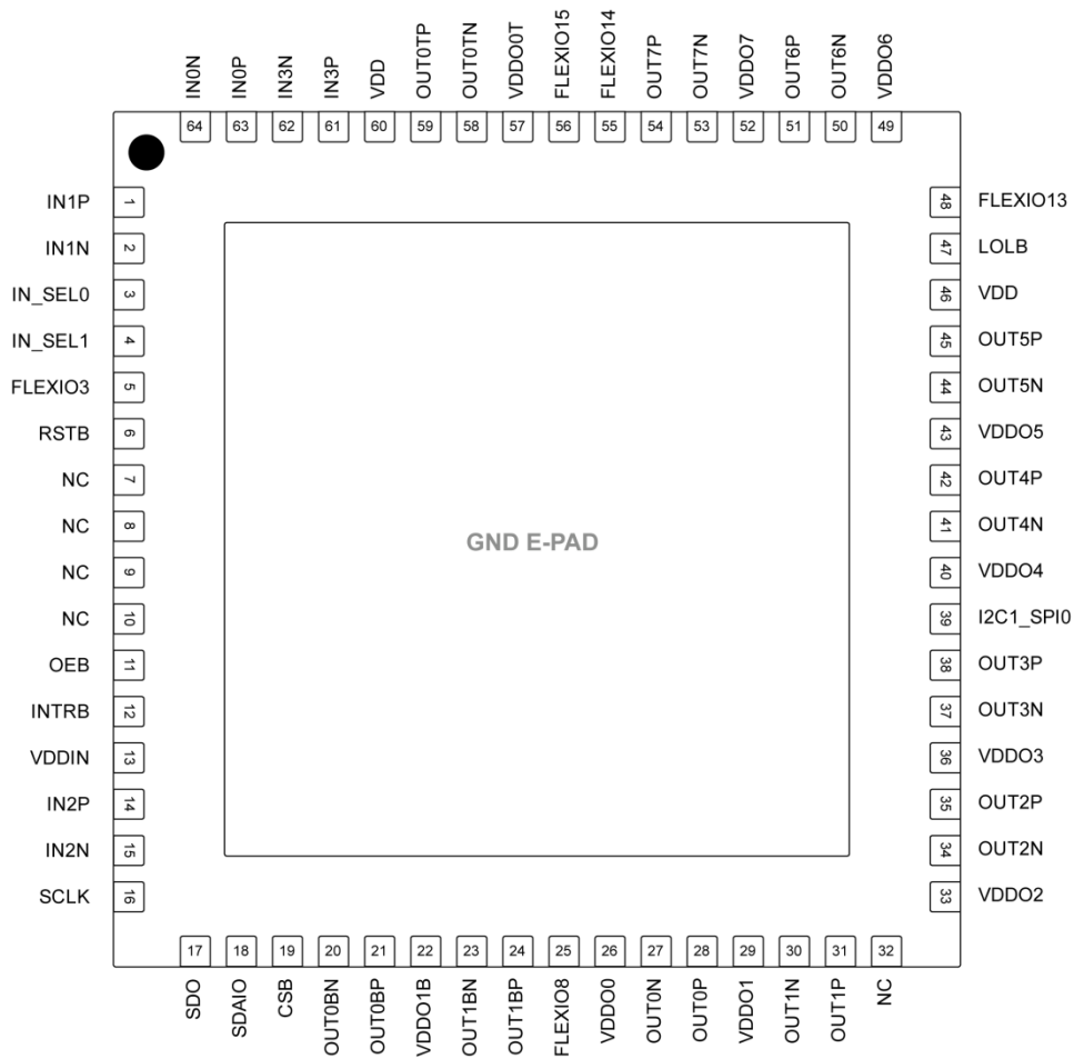
Figure 6. SiT95148 Top View
