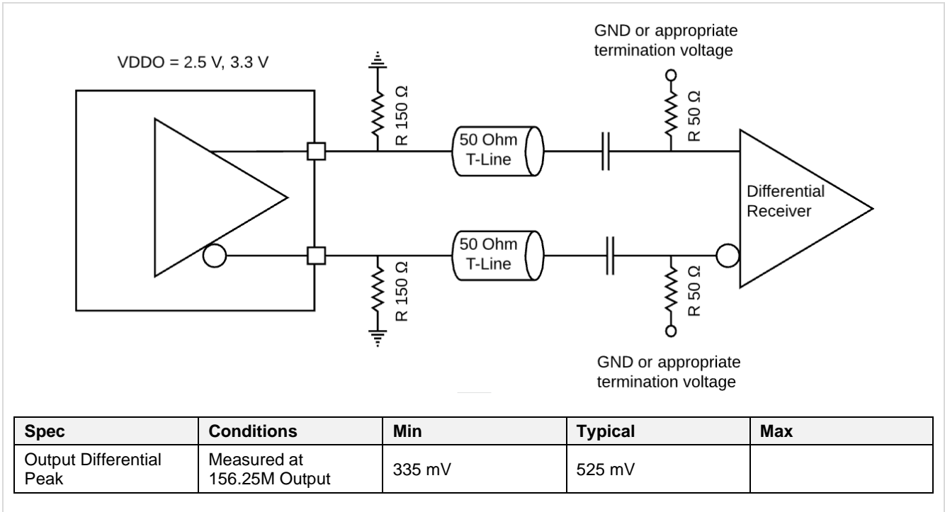
Figure 23. LVPECL2 for the SiT95148 Output Driver with AC Termination at the Load
